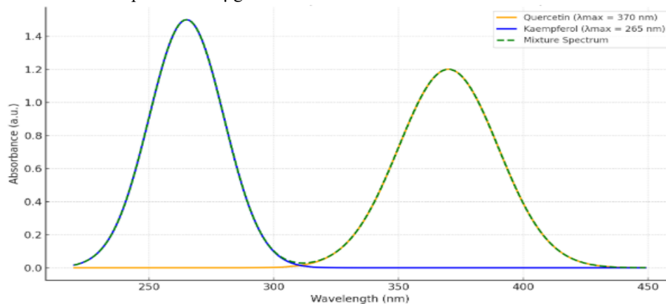
Fig no. 01 Simultaneous graph of Quercetin and kaempferol
